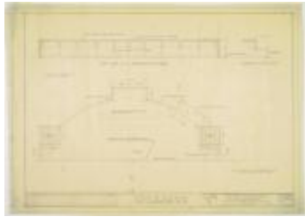
Detail of Platform for Classroom No. 5 (NS090101_000046)
